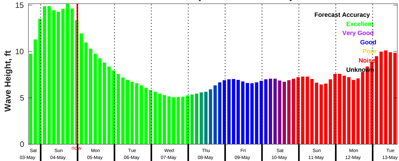
CMEMS Wave Forecast for NDBC 46069 from 03-May-2025 16:00:00 to 13-May-2025 16:00:00
