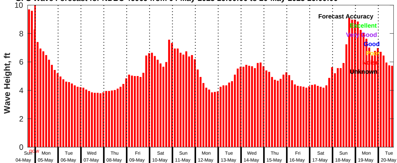
GFS Wave Forecast for NDBC 46069 from 04-May-2025 16:00:00 to 20-May-2025 16:00:00
