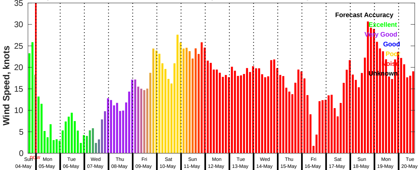
GFS Wind Speed Forecast for NDBC 46069 from 04-May-2025 16:00:00 to 20-May-2025 16:00:00
