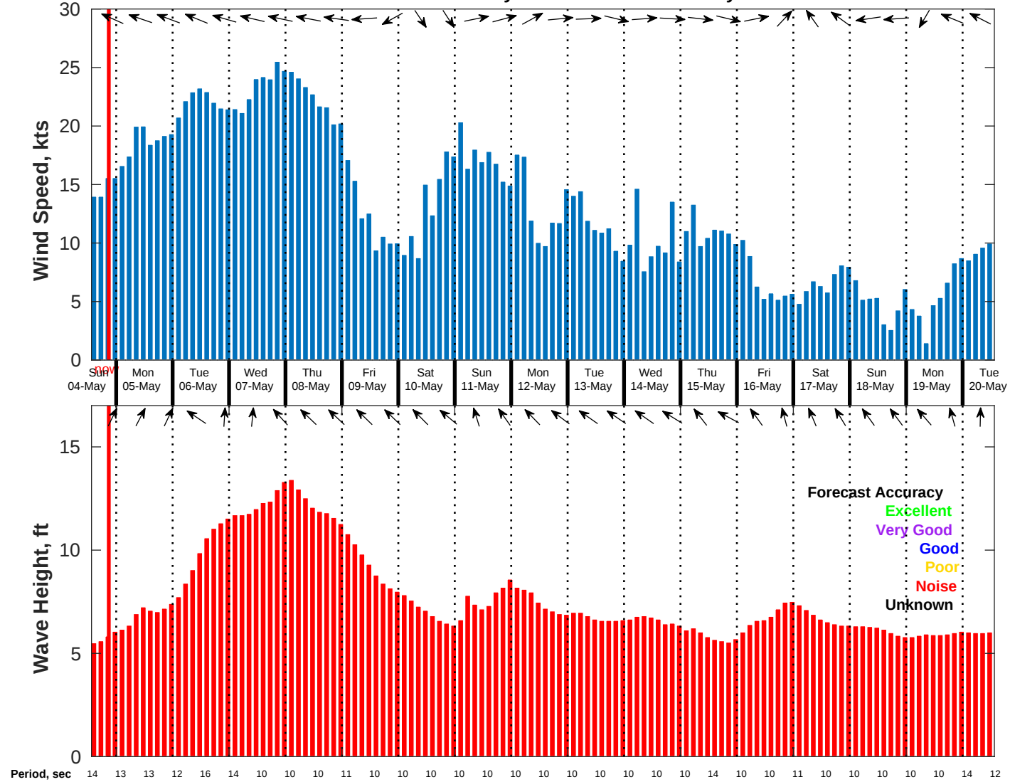
Wind & Wave Forecast for NDBC 51209 from 04-May-2025 13:00:00 to 20-May-2025 13:00:00
