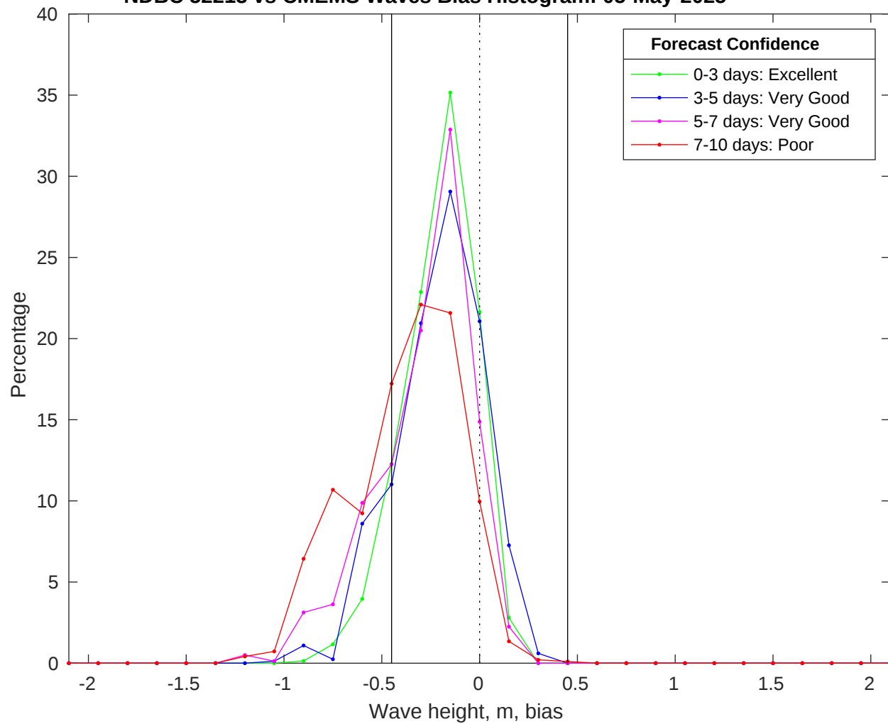
NDBC 52213 vs CMEMS Waves Bias Histogram: 05-May-2025
