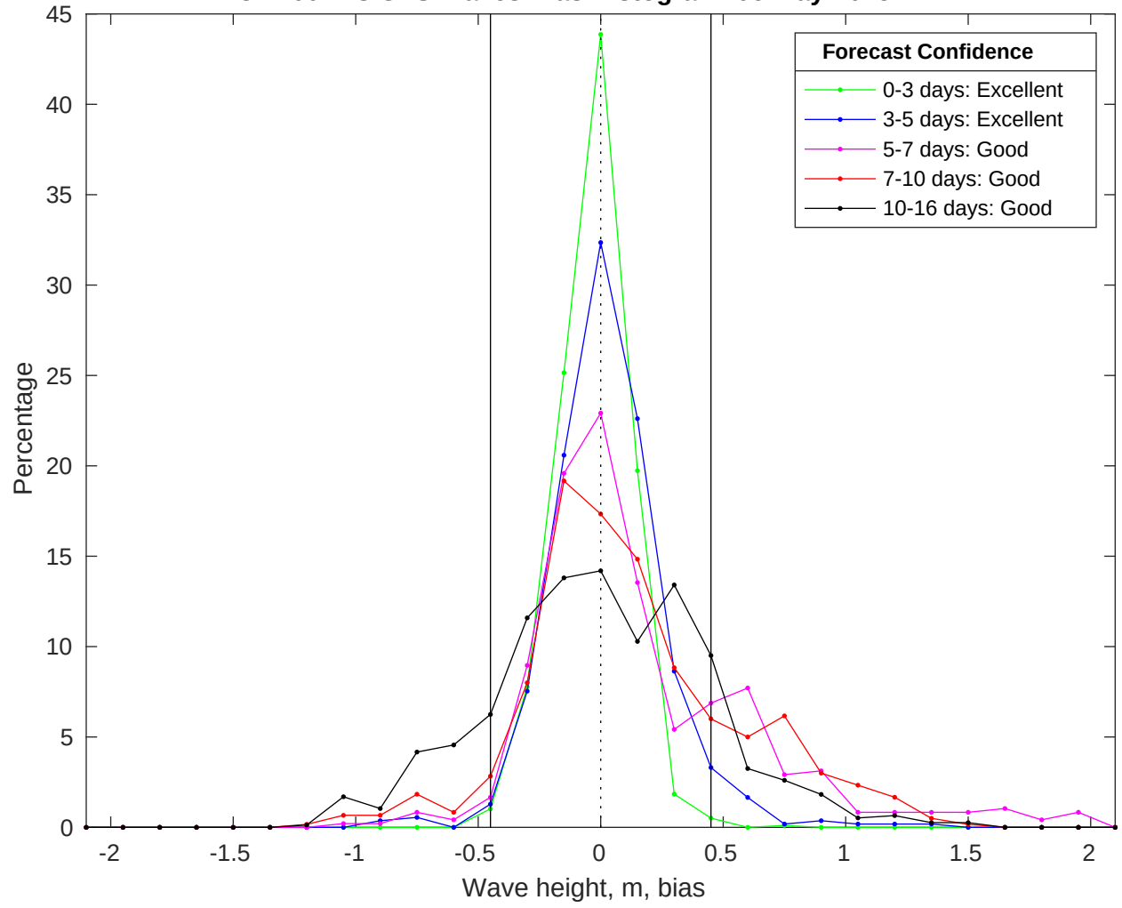
NDBC 41004 vs GFS Waves Bias Histogram: 06-May-2025
