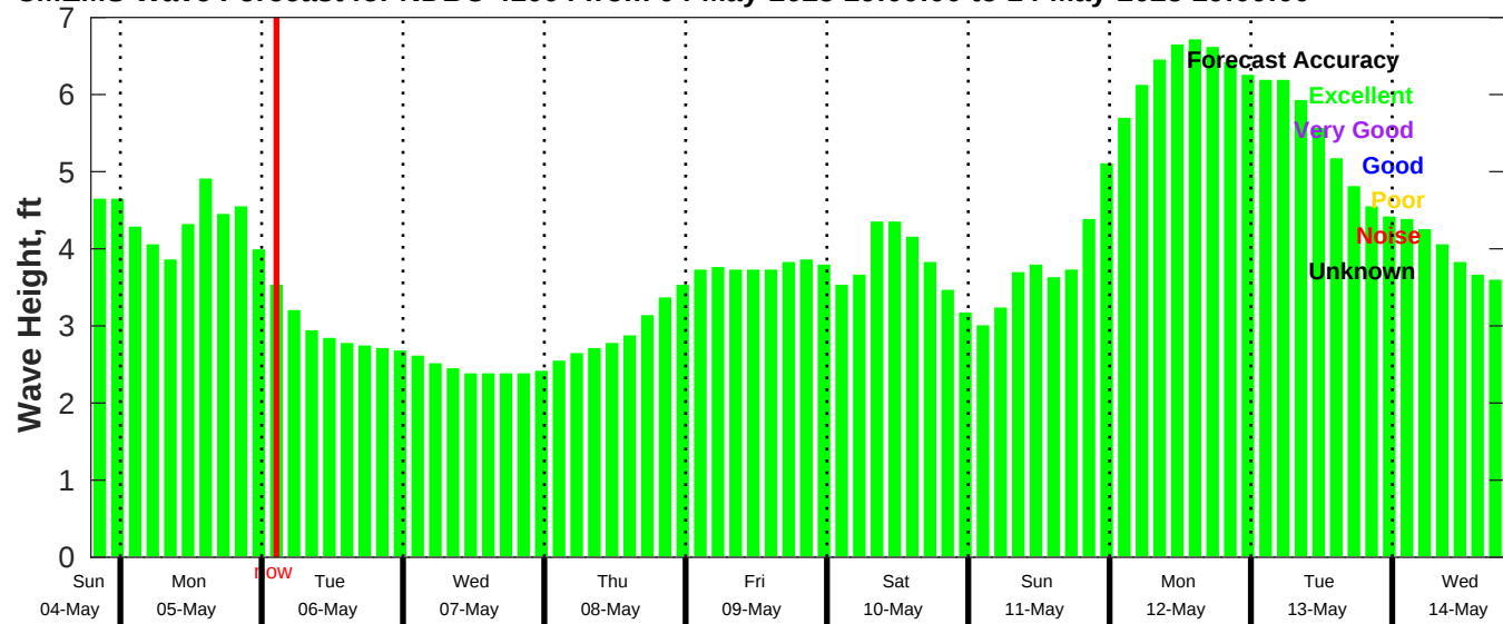
CMEMS Wave Forecast for NDBC 41004 from 04-May-2025 19:00:00 to 14-May-2025 19:00:00
