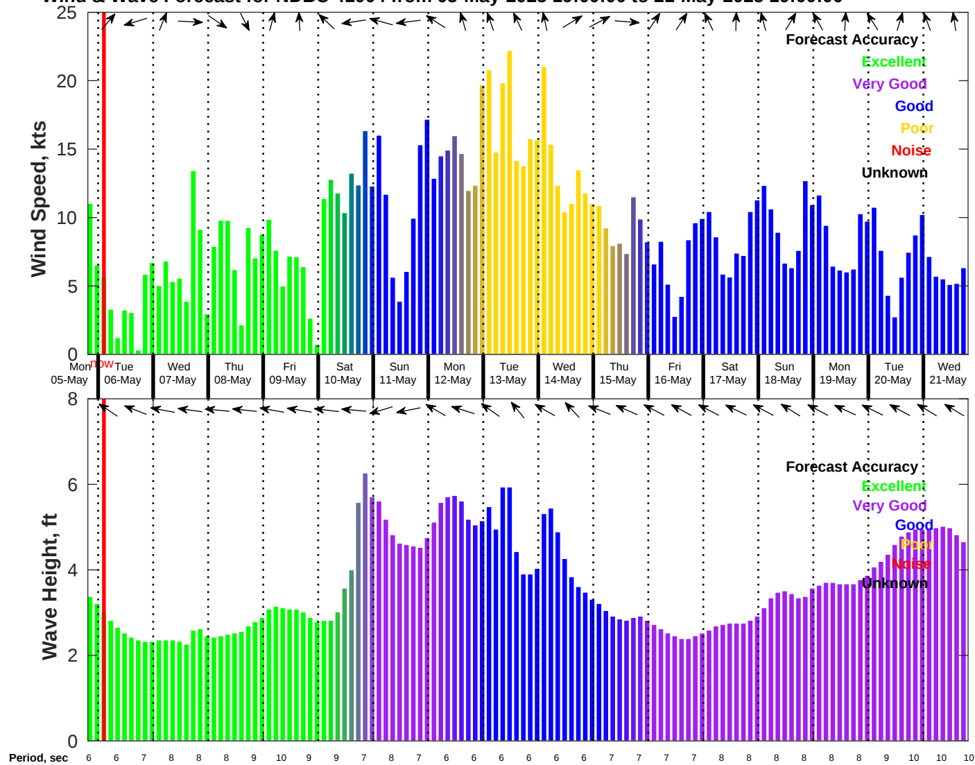
Wind & Wave Forecast for NDBC 41004 from 05-May-2025 19:00:00 to 21-May-2025 19:00:00
