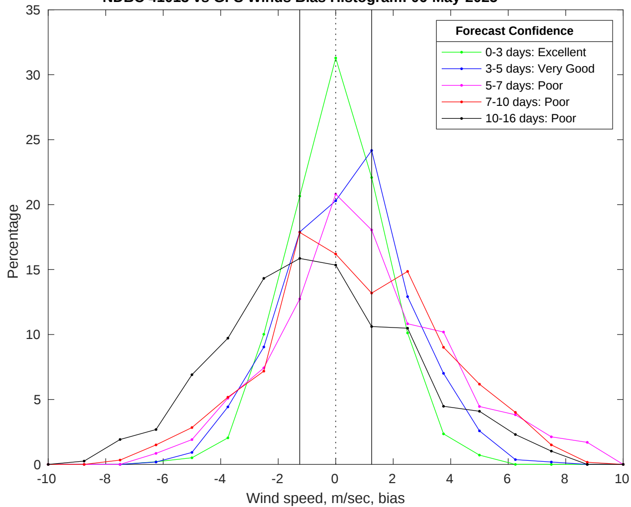
NDBC 41013 vs GFS Winds Bias Histogram: 06-May-2025
