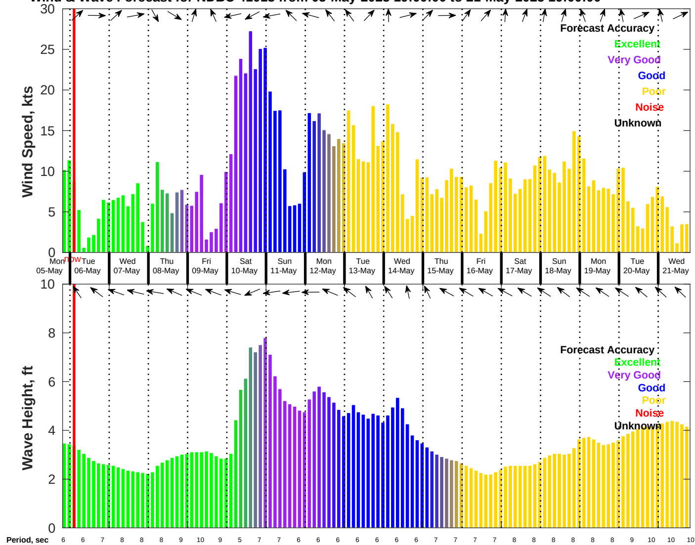
Wind & Wave Forecast for NDBC 41013 from 05-May-2025 19:00:00 to 21-May-2025 19:00:00
