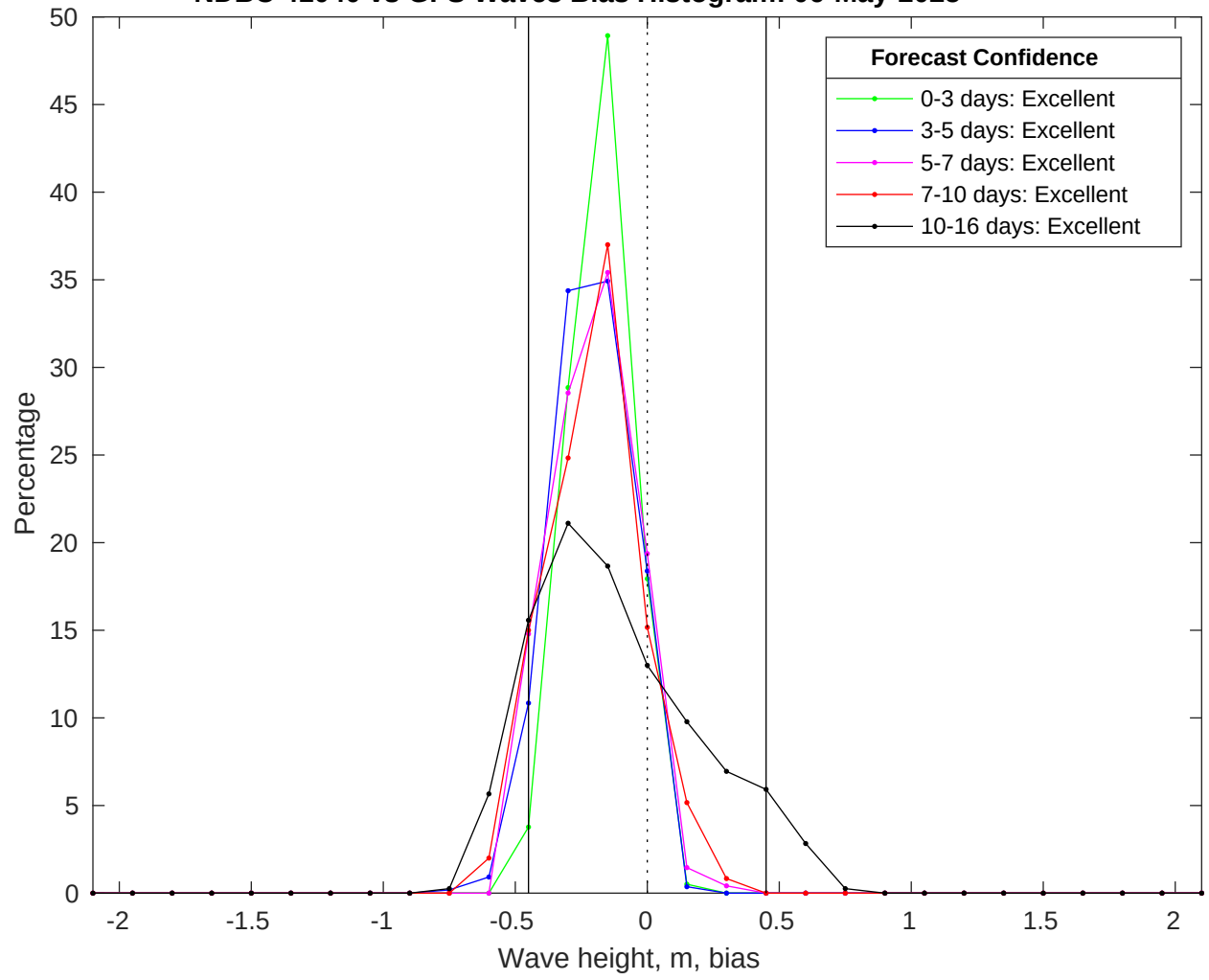
NDBC 41040 vs GFS Waves Bias Histogram: 06-May-2025
