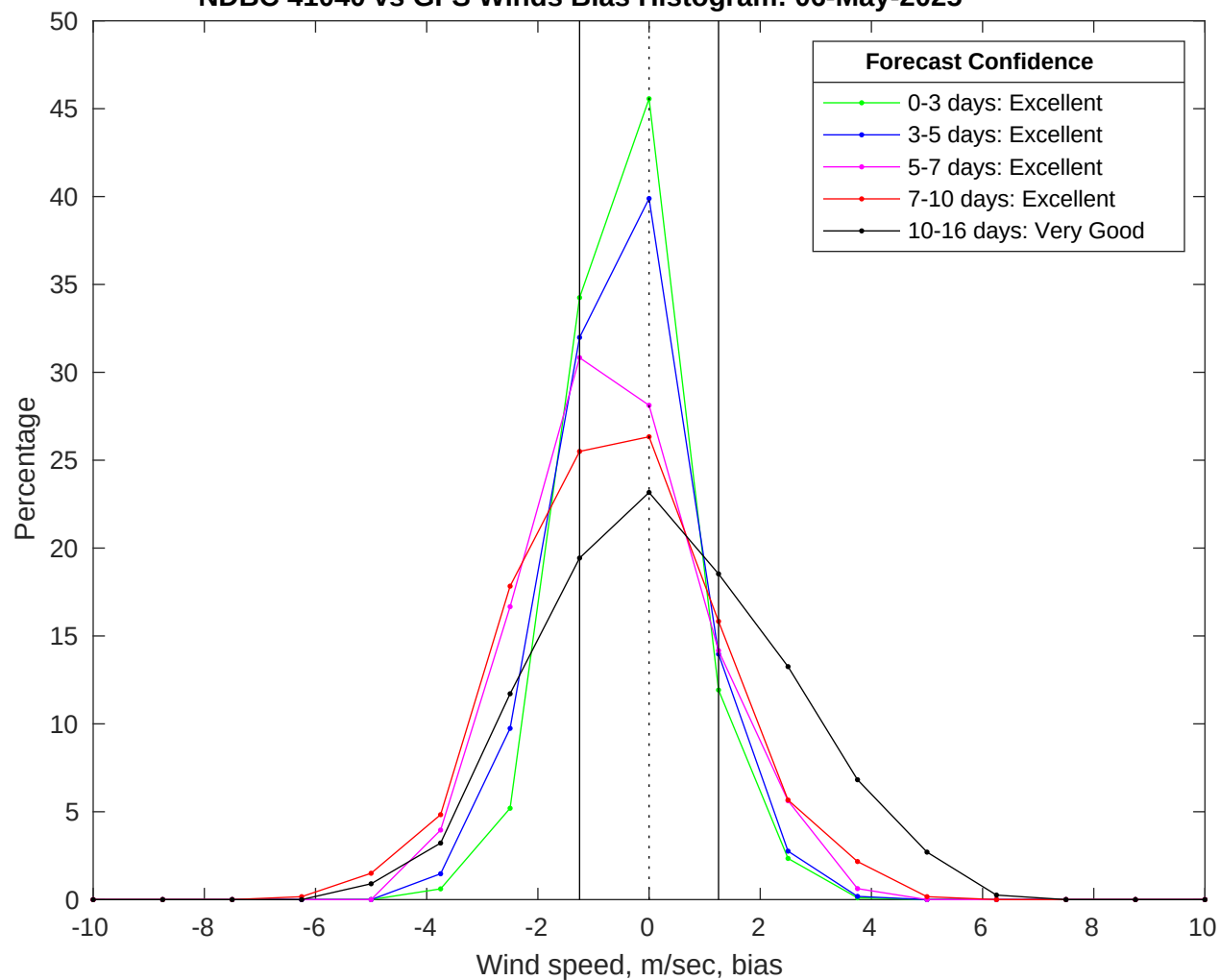
NDBC 41040 vs GFS Winds Bias Histogram: 06-May-2025
