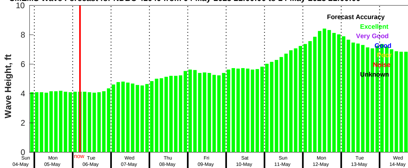
CMEMS Wave Forecast for NDBC 41040 from 04-May-2025 21:00:00 to 14-May-2025 21:00:00
