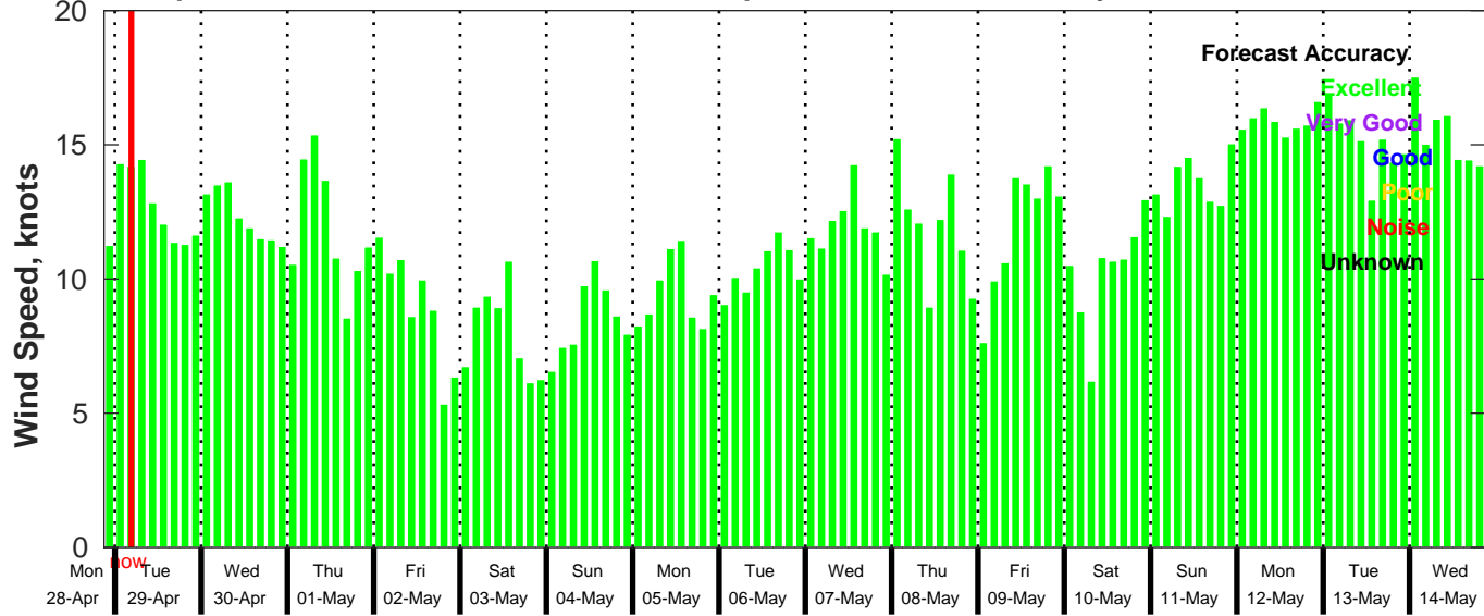
GFS Wind Speed Forecast for NDBC 41040 from 28-Apr-2025 21:00:00 to 14-May-2025 21:00:00
