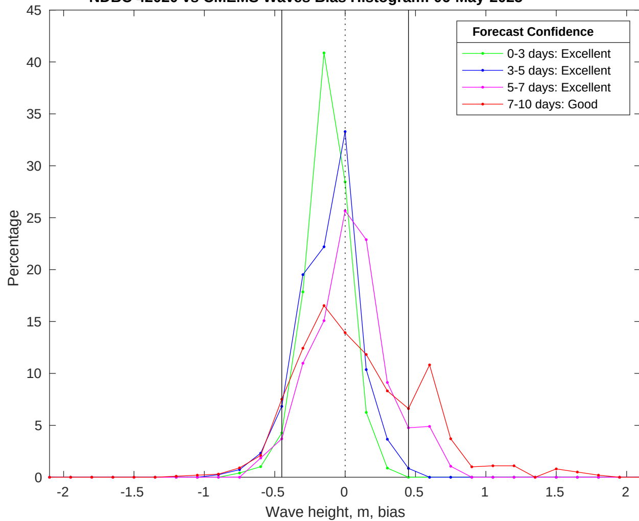
NDBC 42020 vs CMEMS Waves Bias Histogram: 06-May-2025
