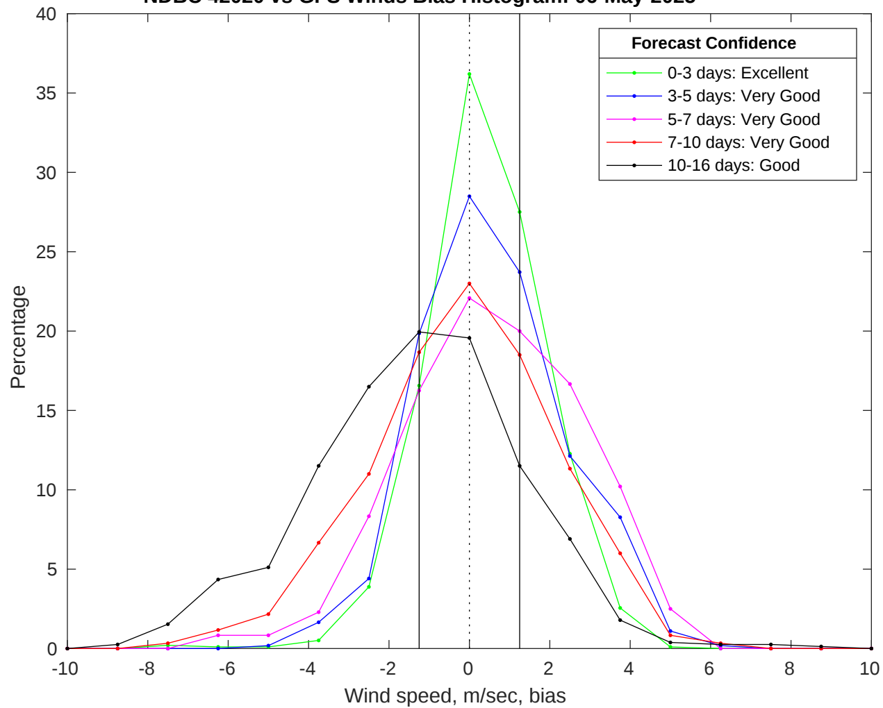
NDBC 42020 vs GFS Winds Bias Histogram: 06-May-2025
