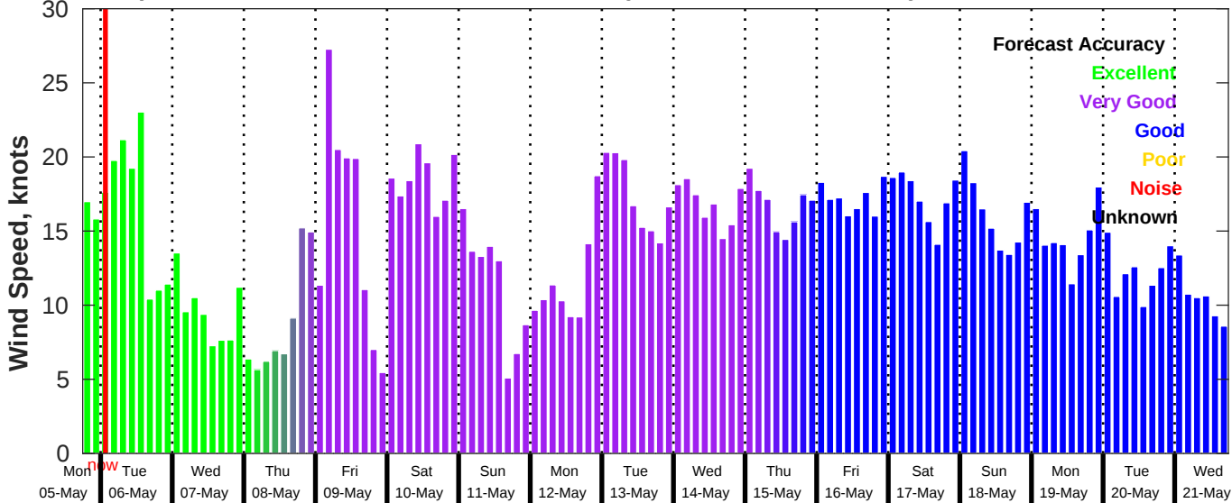
GFS Wind Speed Forecast for NDBC 42020 from 05-May-2025 18:00:00 to 21-May-2025 18:00:00
