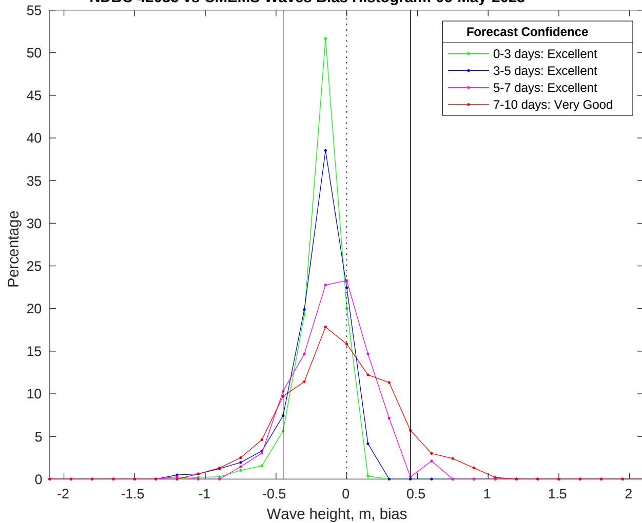
NDBC 42035 vs CMEMS Waves Bias Histogram: 06-May-2025
