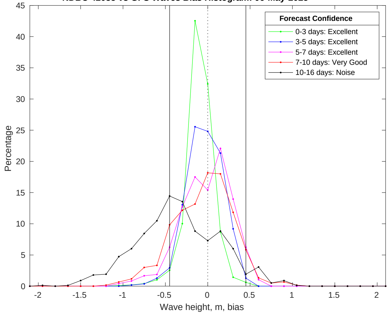
NDBC 42035 vs GFS Waves Bias Histogram: 06-May-2025
