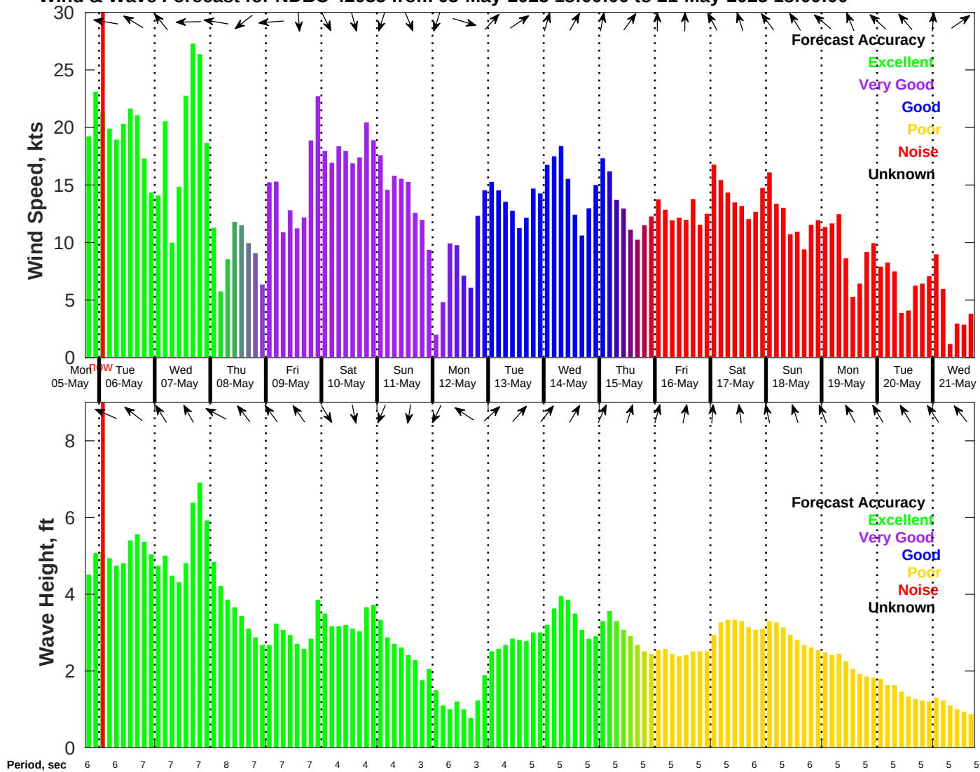
Wind & Wave Forecast for NDBC 42035 from 05-May-2025 18:00:00 to 21-May-2025 18:00:00
