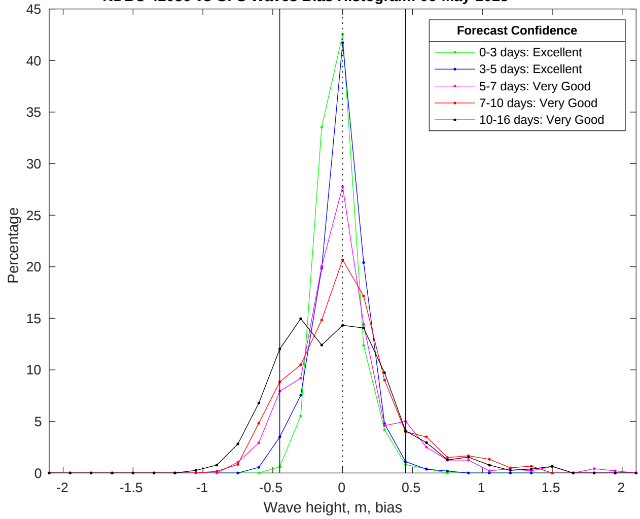
NDBC 42036 vs GFS Waves Bias Histogram: 06-May-2025
