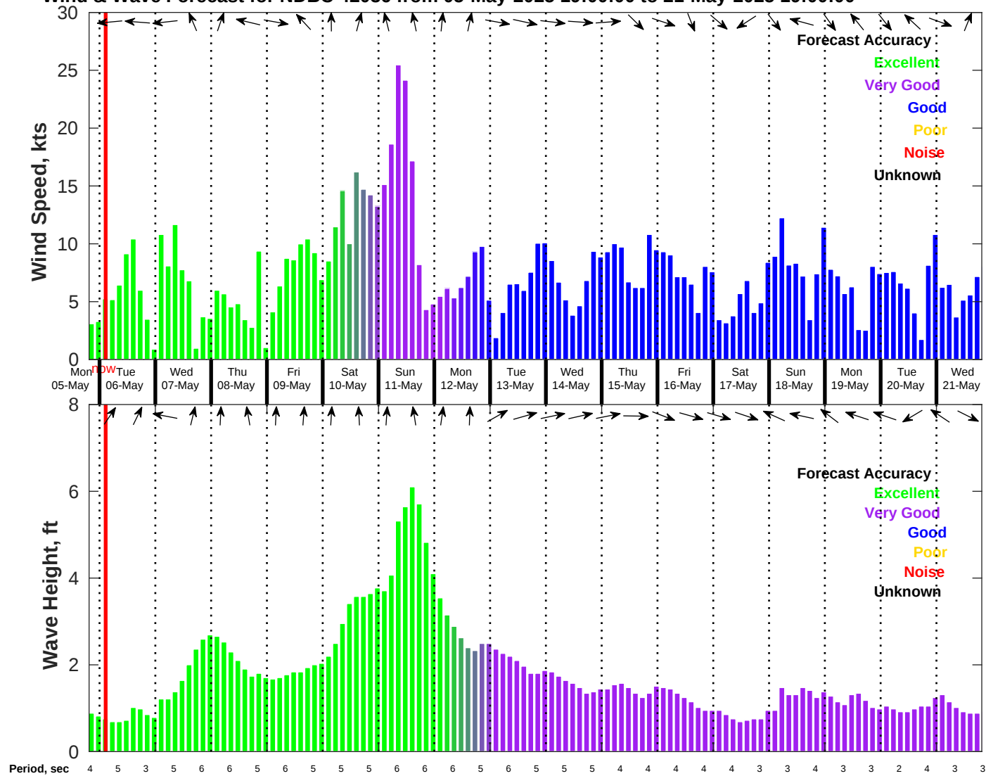
Wind & Wave Forecast for NDBC 42036 from 05-May-2025 19:00:00 to 21-May-2025 19:00:00
