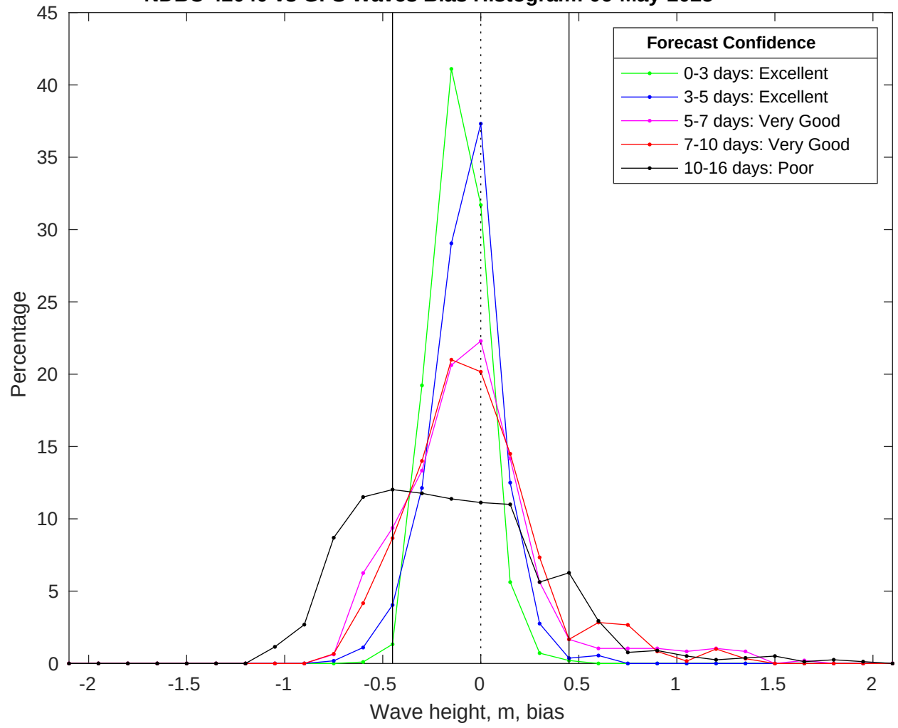
NDBC 42040 vs GFS Waves Bias Histogram: 06-May-2025
