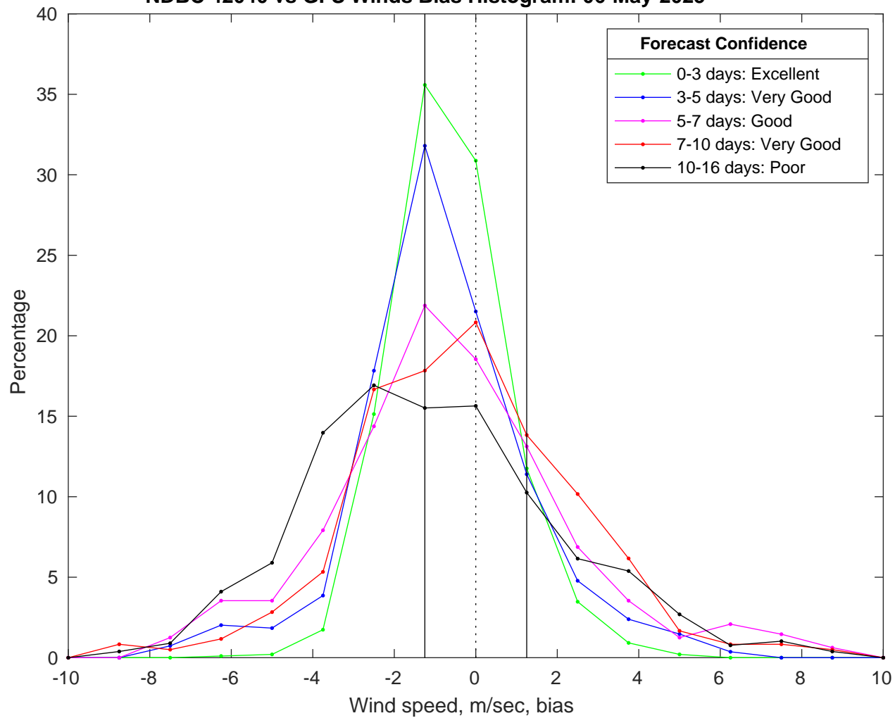
NDBC 42040 vs GFS Winds Bias Histogram: 06-May-2025
