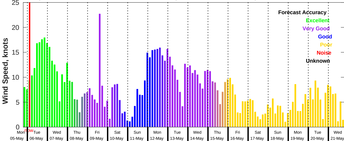
GFS Wind Speed Forecast for NDBC 42040 from 05-May-2025 19:00:00 to 21-May-2025 19:00:00
