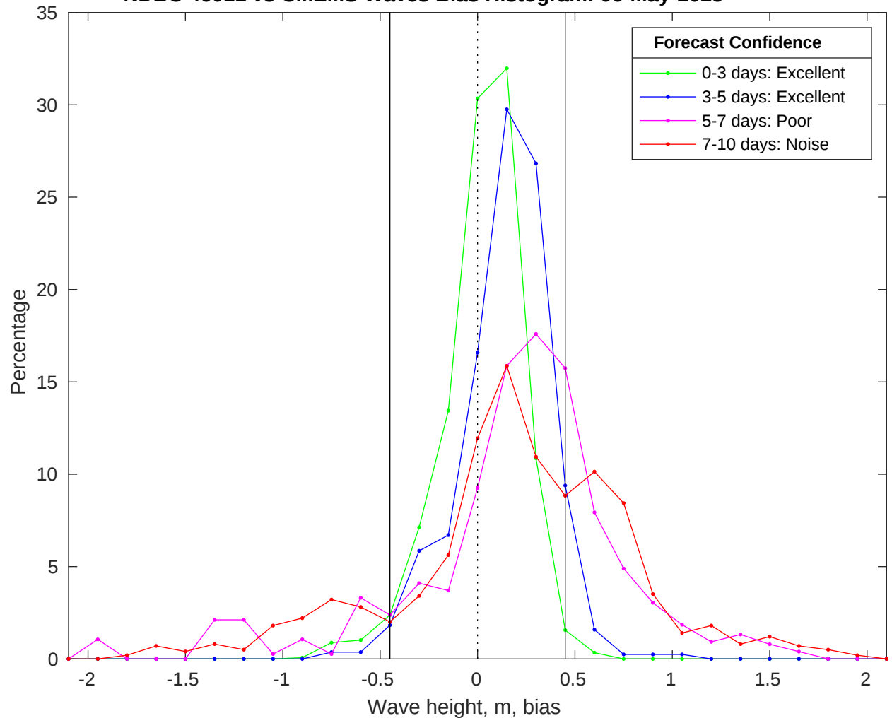
NDBC 46011 vs CMEMS Waves Bias Histogram: 06-May-2025
