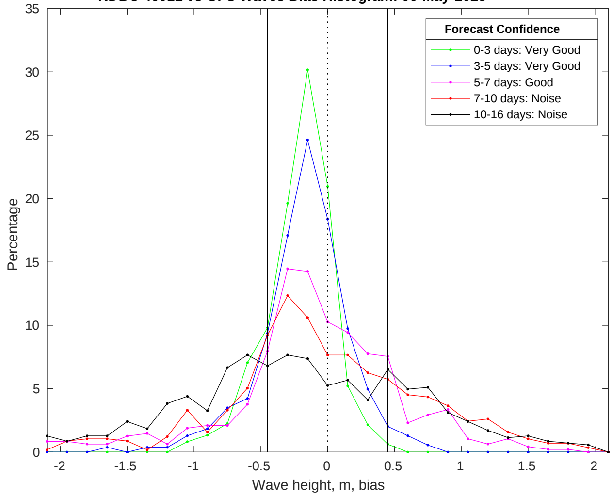
NDBC 46011 vs GFS Waves Bias Histogram: 06-May-2025
