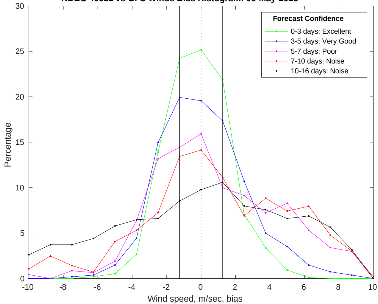
NDBC 46011 vs GFS Winds Bias Histogram: 06-May-2025
