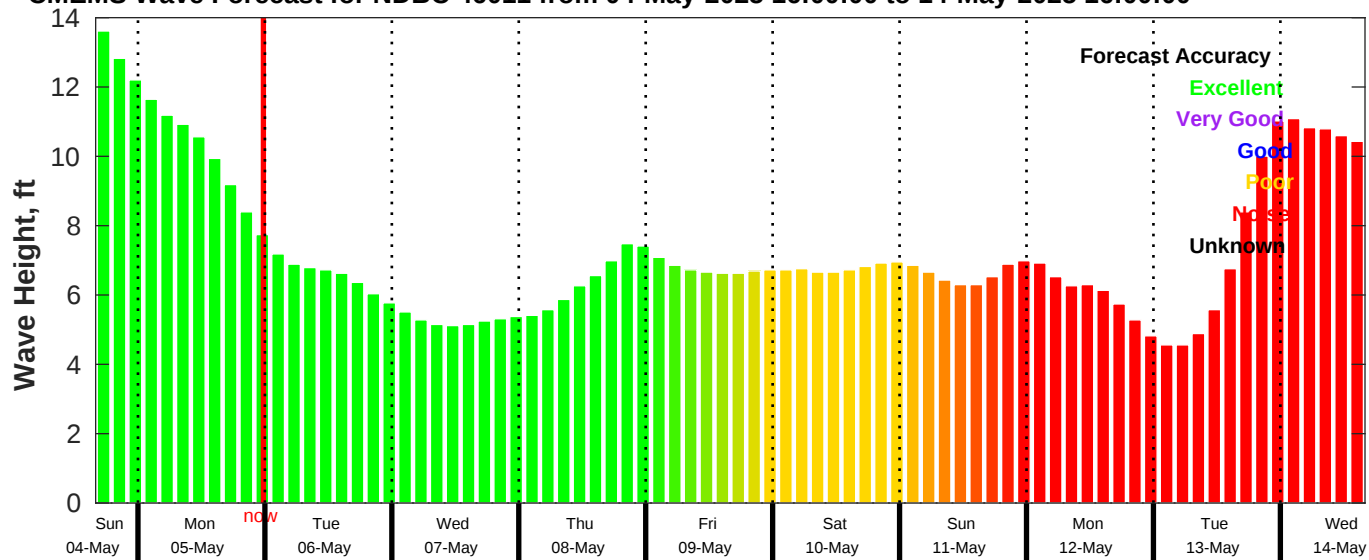
CMEMS Wave Forecast for NDBC 46011 from 04-May-2025 16:00:00 to 14-May-2025 16:00:00
