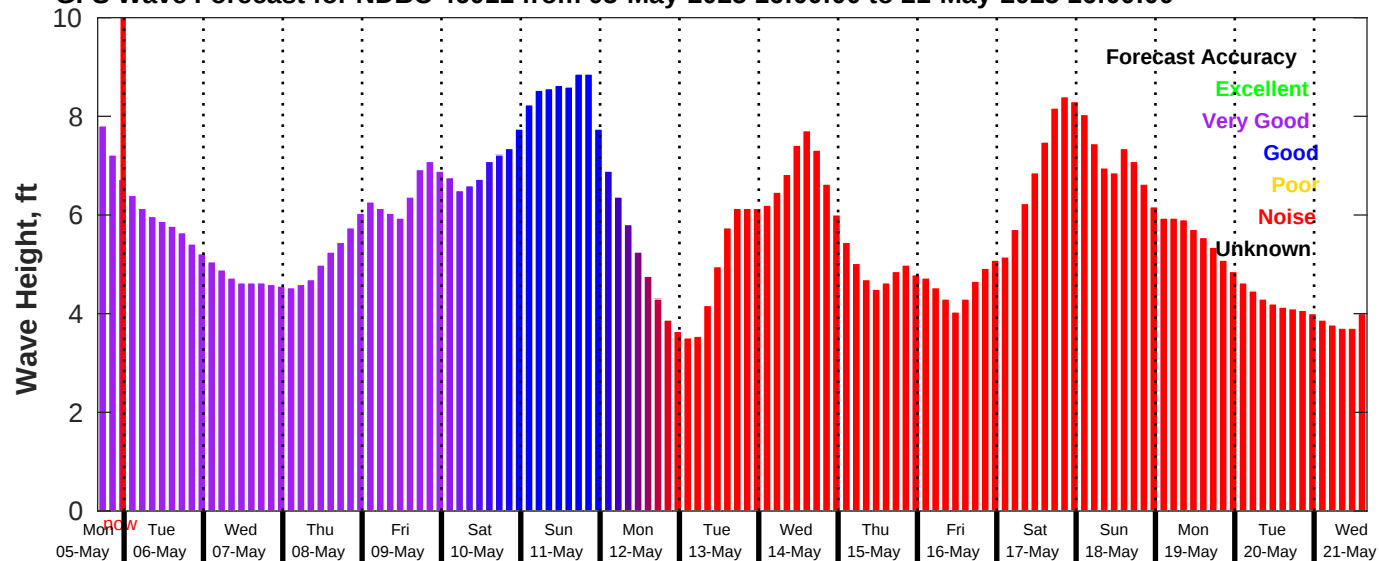
GFS Wave Forecast for NDBC 46011 from 05-May-2025 16:00:00 to 21-May-2025 16:00:00
