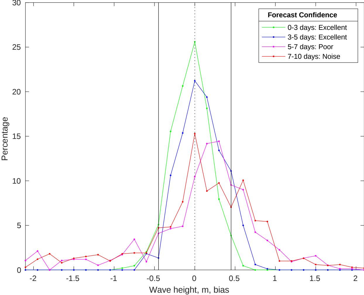
NDBC 46028 vs CMEMS Waves Bias Histogram: 06-May-2025
