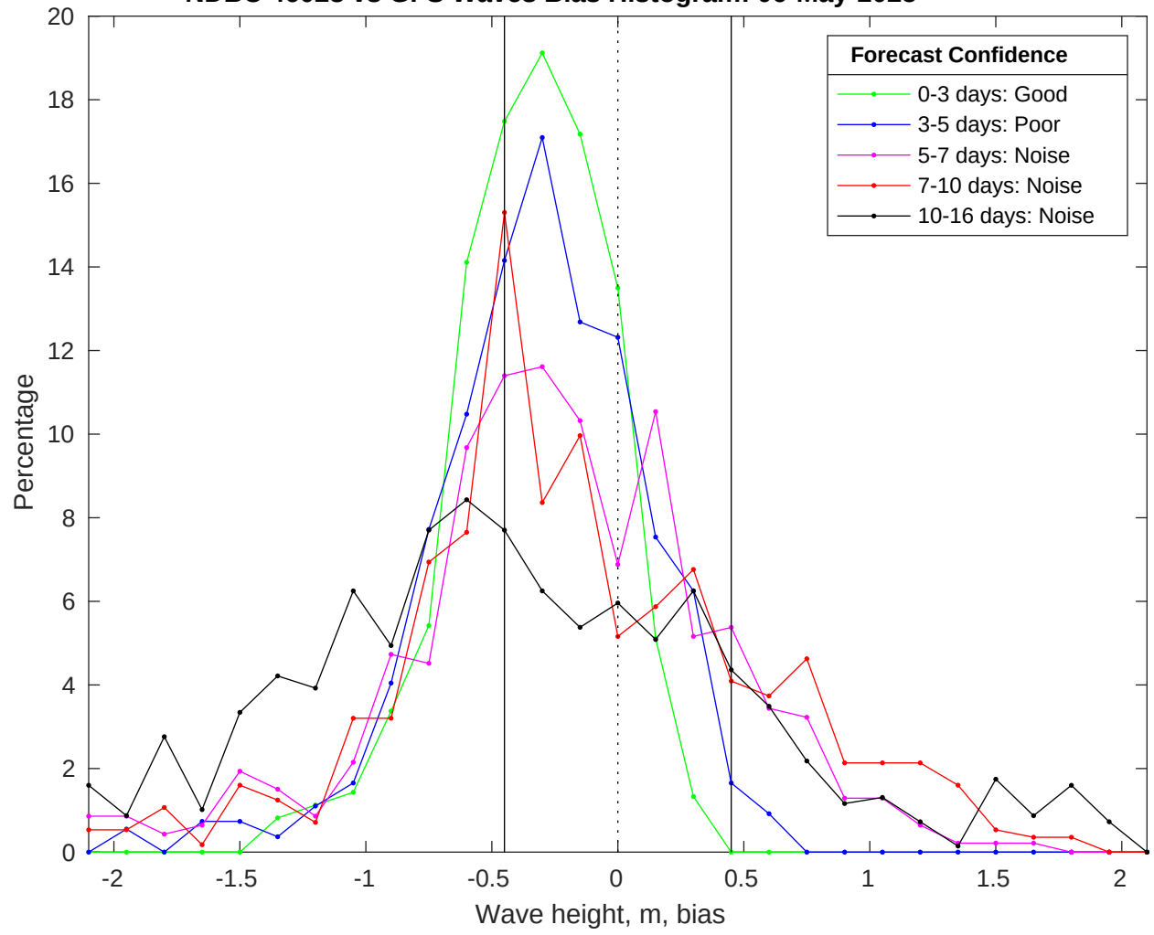
NDBC 46028 vs GFS Waves Bias Histogram: 06-May-2025
