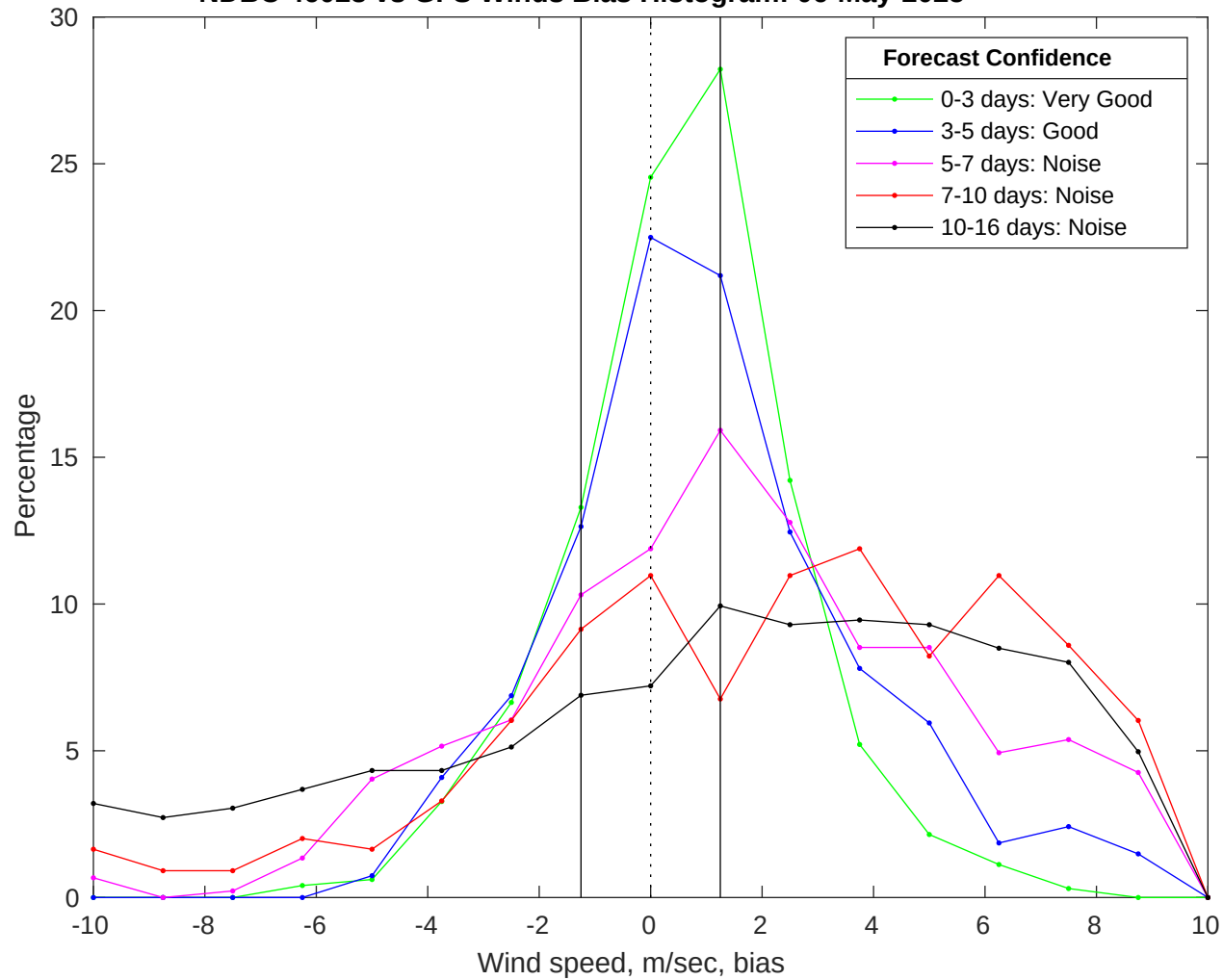
NDBC 46028 vs GFS Winds Bias Histogram: 06-May-2025
