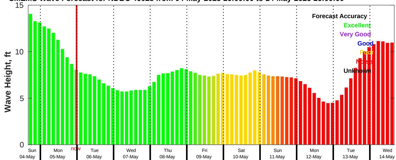
CMEMS Wave Forecast for NDBC 46028 from 04-May-2025 16:00:00 to 14-May-2025 16:00:00
