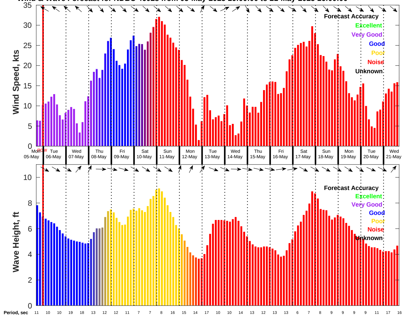
Wind & Wave Forecast for NDBC 46028 from 05-May-2025 16:00:00 to 21-May-2025 16:00:00
