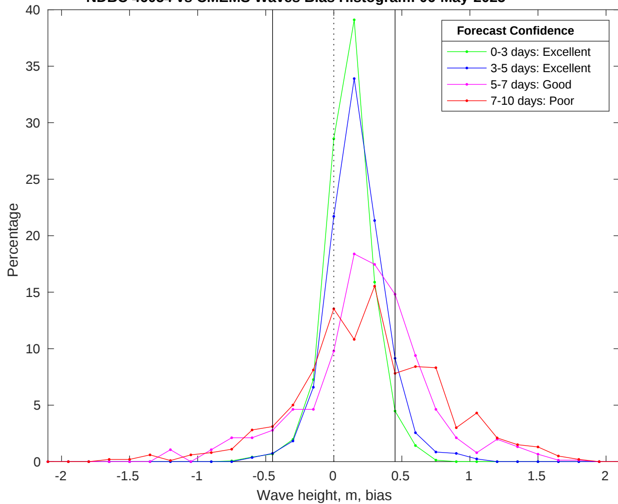
NDBC 46054 vs CMEMS Waves Bias Histogram: 06-May-2025
