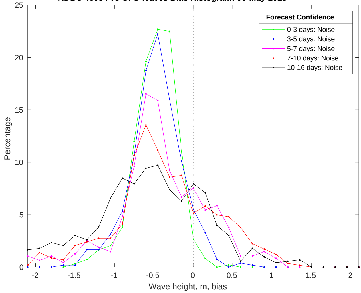
NDBC 46054 vs GFS Waves Bias Histogram: 06-May-2025
