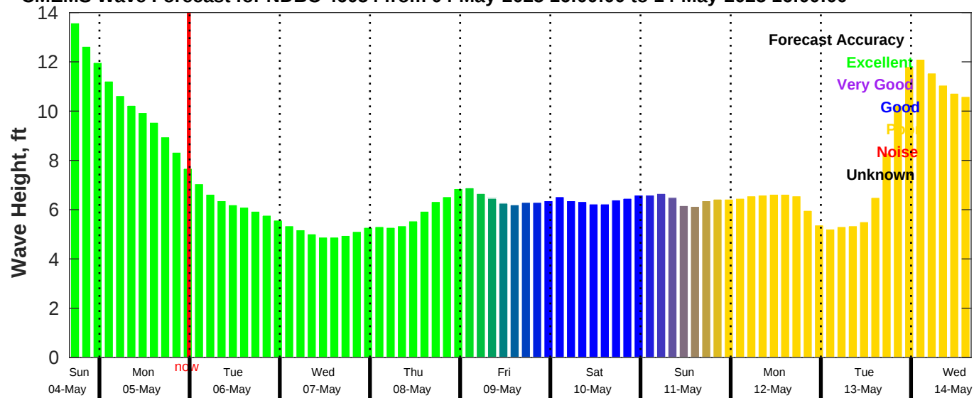
CMEMS Wave Forecast for NDBC 46054 from 04-May-2025 16:00:00 to 14-May-2025 16:00:00
