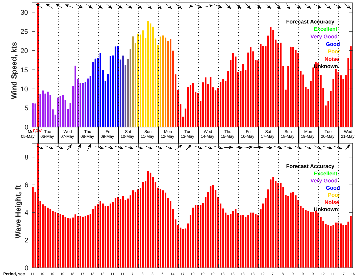
Wind & Wave Forecast for NDBC 46054 from 05-May-2025 16:00:00 to 21-May-2025 16:00:00
