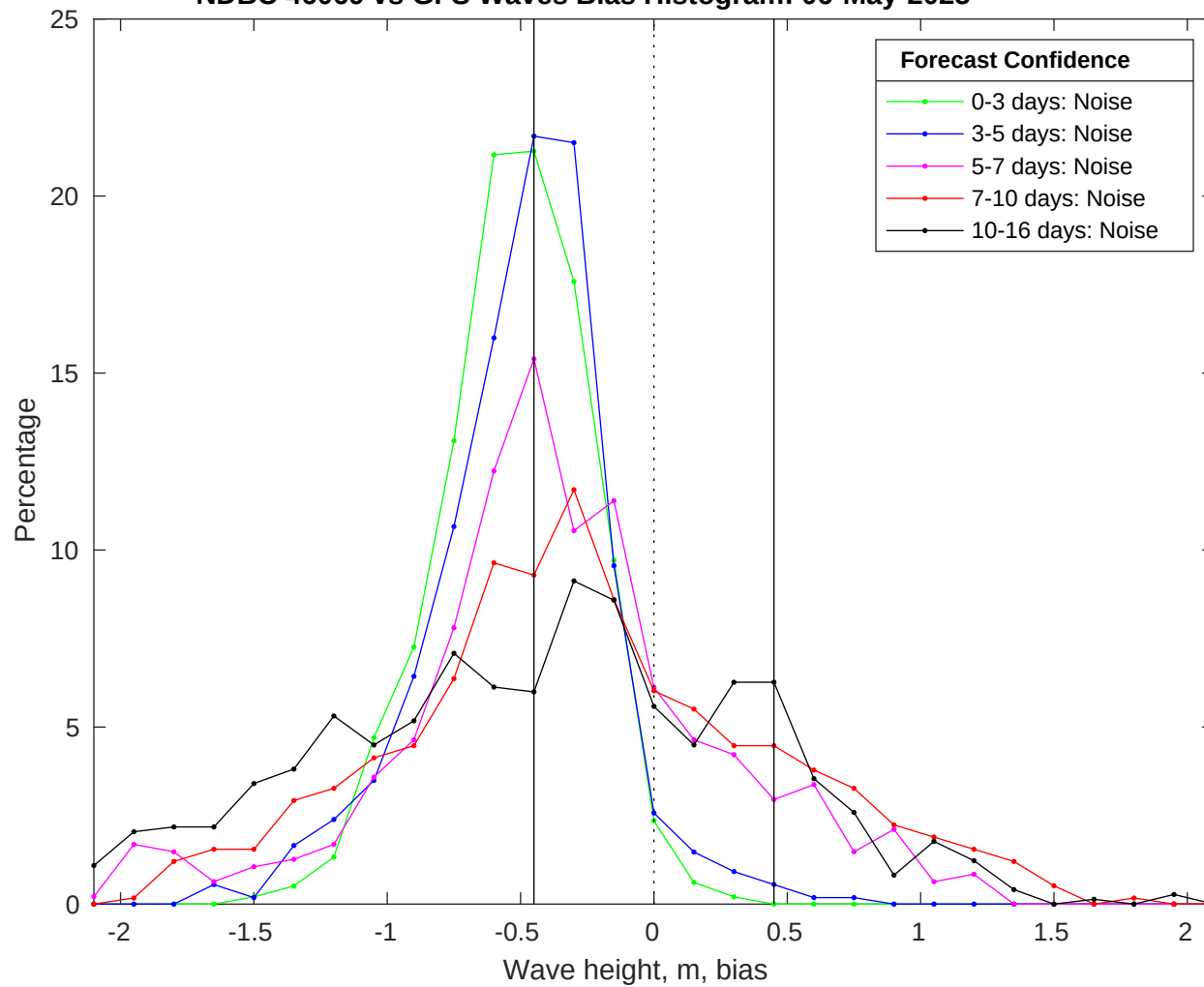
NDBC 46069 vs GFS Waves Bias Histogram: 06-May-2025
