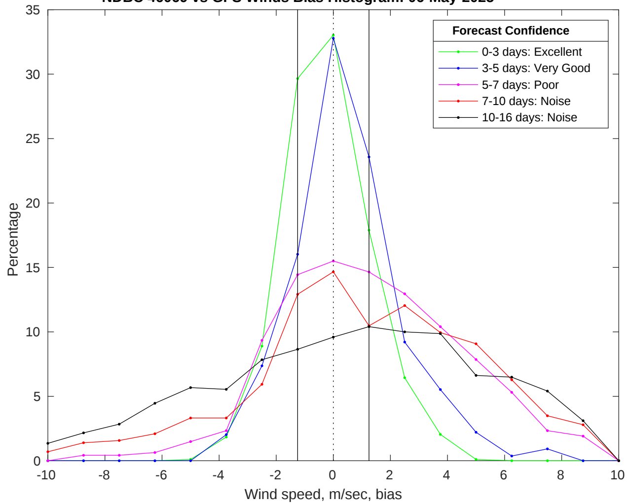
NDBC 46069 vs GFS Winds Bias Histogram: 06-May-2025
