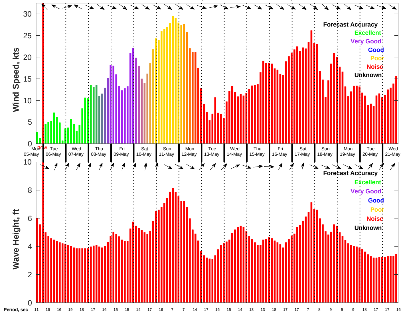
Wind & Wave Forecast for NDBC 46069 from 05-May-2025 16:00:00 to 21-May-2025 16:00:00
