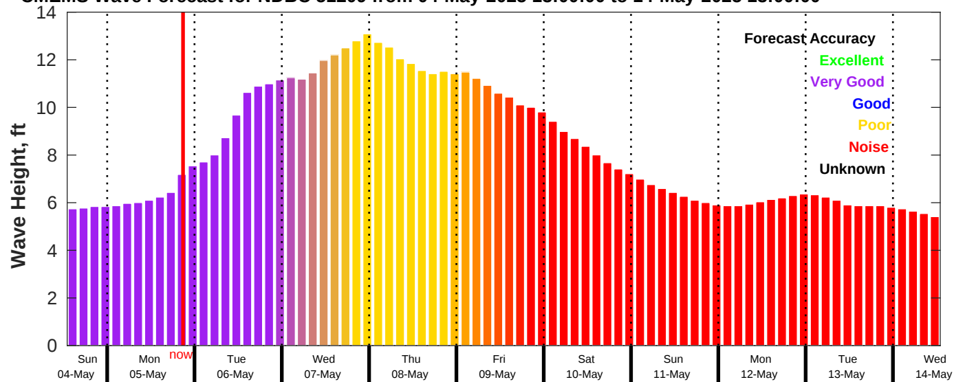
CMEMS Wave Forecast for NDBC 51209 from 04-May-2025 13:00:00 to 14-May-2025 13:00:00
