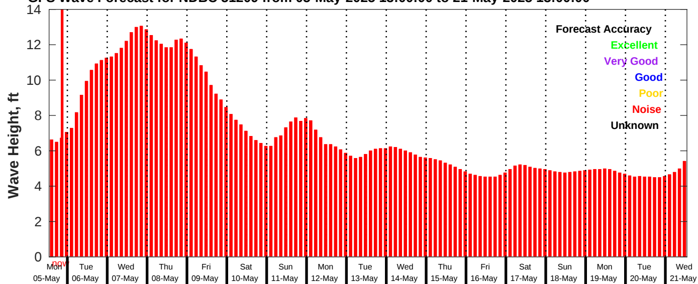
GFS Wave Forecast for NDBC 51209 from 05-May-2025 13:00:00 to 21-May-2025 13:00:00
