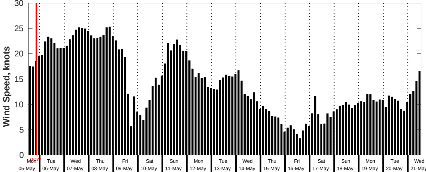
GFS Wind Speed Forecast for NDBC 51209 from 05-May-2025 13:00:00 to 21-May-2025 13:00:00
