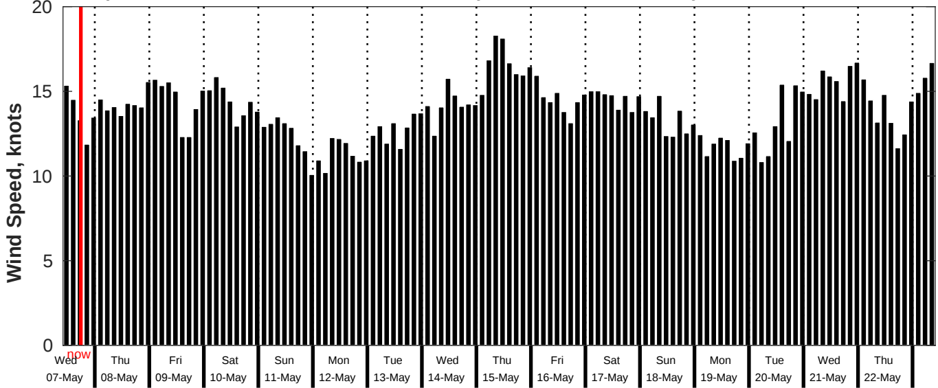
GFS Wind Speed Forecast for NDBC 52211 from 06-May-2025 10:00:00 to 22-May-2025 10:00:00
