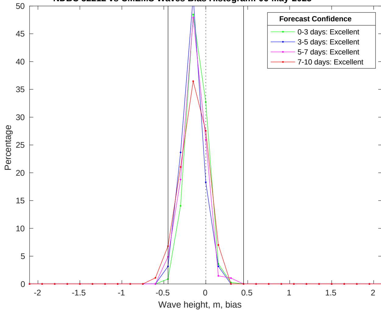
NDBC 52212 vs CMEMS Waves Bias Histogram: 06-May-2025
