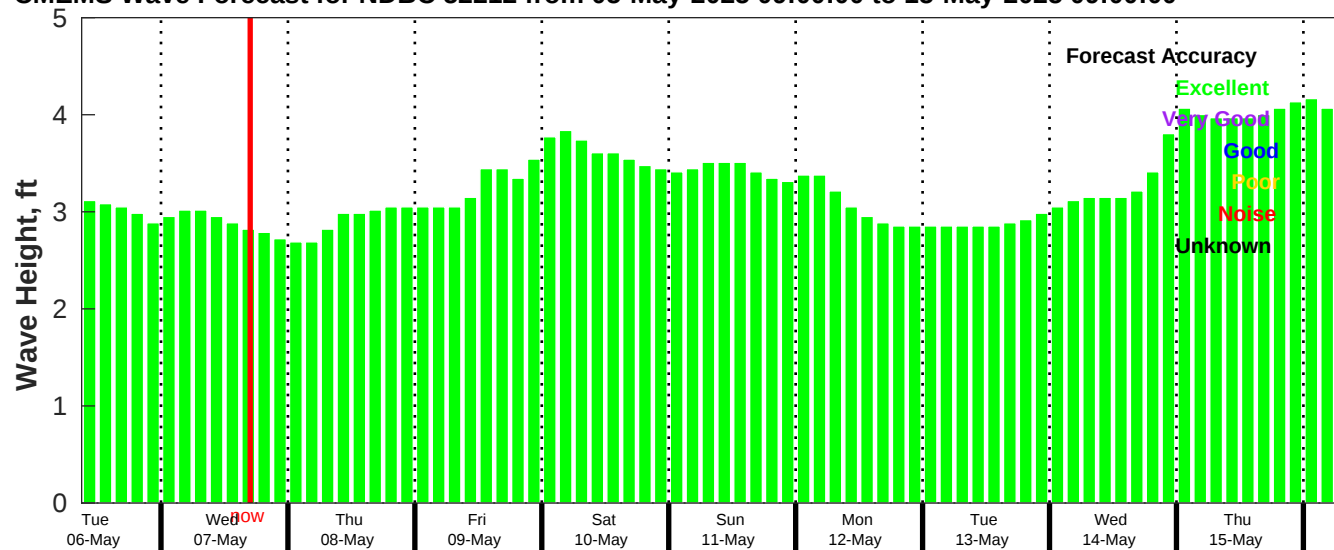
CMEMS Wave Forecast for NDBC 52212 from 05-May-2025 09:00:00 to 15-May-2025 09:00:00
