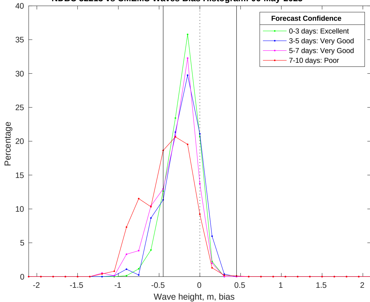
NDBC 52213 vs CMEMS Waves Bias Histogram: 06-May-2025
