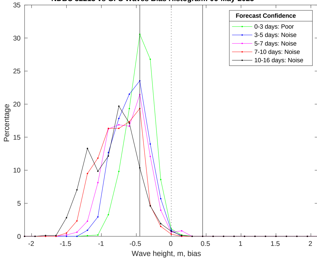
NDBC 52213 vs GFS Waves Bias Histogram: 06-May-2025
